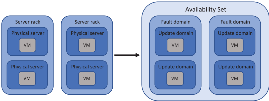
Figure 7.4 Hardware in an Azure data center is logically divided into update domains and fault domains. These logical domains allow the Azure platform to understand how to distribute your VMs across the underlying hardware to meet your redundancy requirements. This example is basic: an update domain likely contains more than one physical server.
